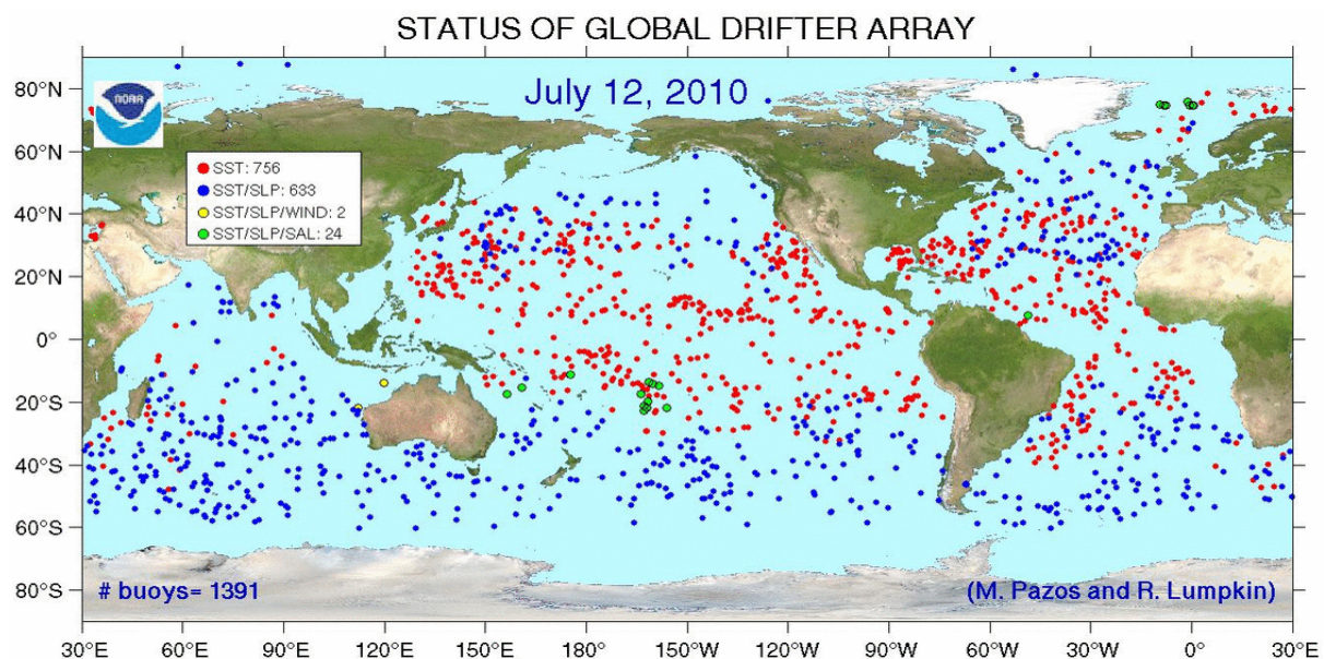
Figure 9: The distribution of drifting buoys as of July 2010 (Source: http://www.aomi.noaa.gov/phod/graphics/dacdata/globpop.gif ).
