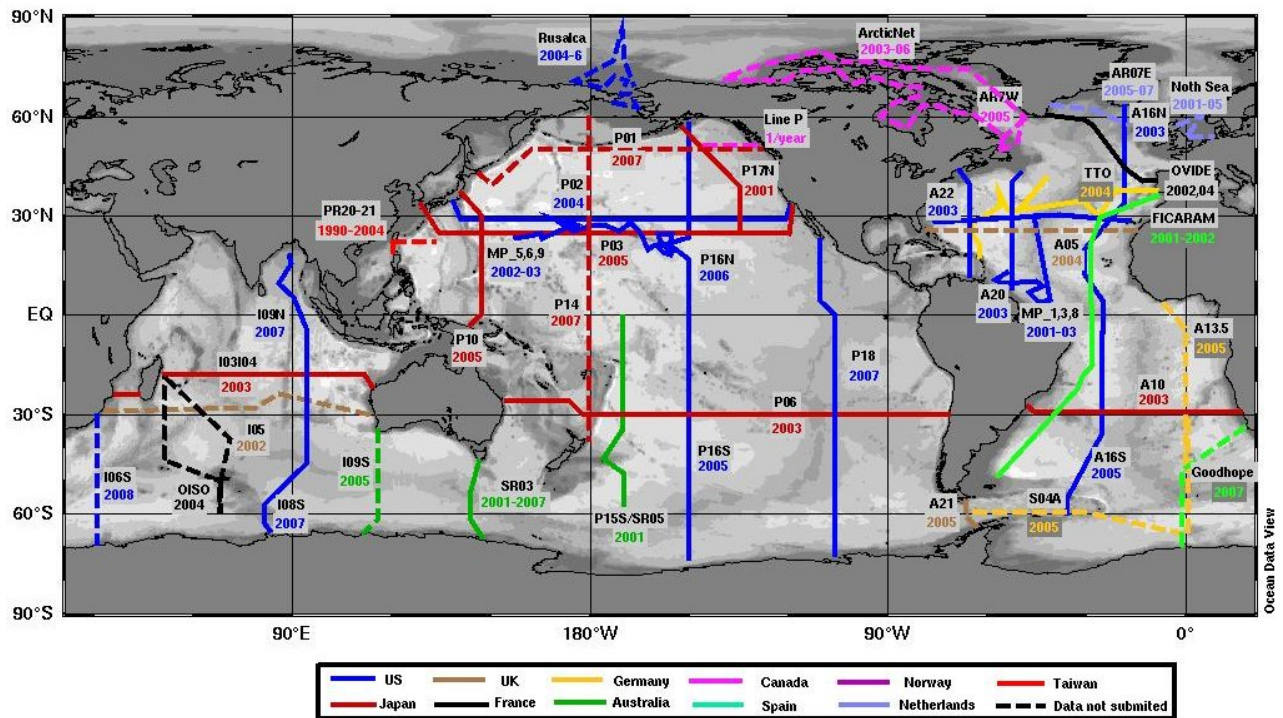
Figure 11: Map of completed International Repeat Hydrography Program sections, with colours indicating the country responsible. The dashed lines indicate data not submitted to the internationally-agreed data archive. 83 Data from certain hydrographic lines led by scientists from nearly all the countries involved in the Program have not yet been submitted to the international data archive.
