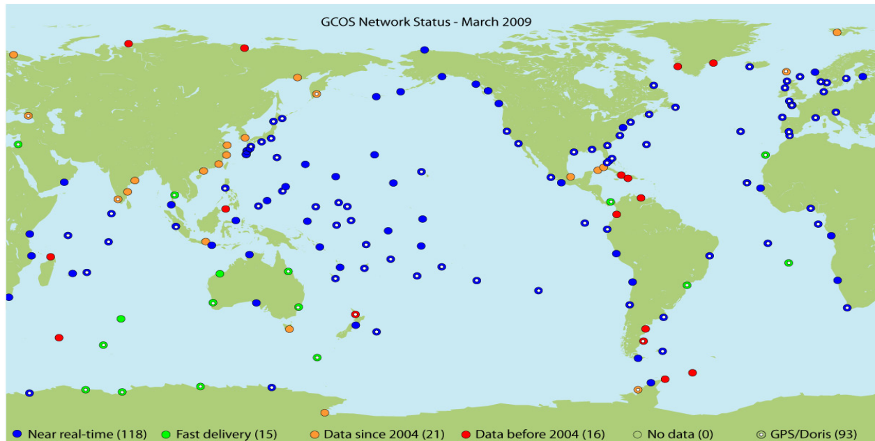
Figure 10: Sea-level gauges in the GCOS subset of the GLOSS Core Network. "Near real-time" and "Fast Delivery" stations provide high-frequency sea level (hourly or better reports) which are necessary for understanding of sea-level variability in addition to mean sea-level rise. Near real-time stations (blue) provide data typically within 1 hour of collection; Fast delivery (green) within one month. Delayed-mode data within 5 years (orange) or greater (red) include monthly averages provided to the Permanent Service for Mean Sea Level (PSMSL). White dots are placed on tide gauges that are geo-referenced, measuring local land movements, in order to measure absolute sea-level change.
